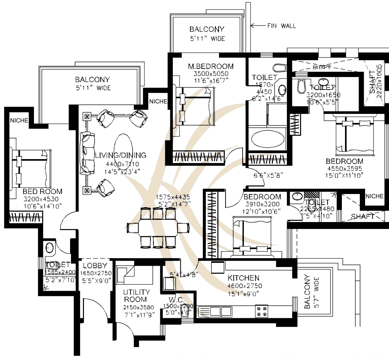
TENTATIVE PLAN OF APARTMENT NO. 1 & 3 IN BLOCKS - J, K, L, M & N
