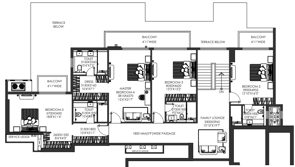
APARTMENT NO. 4 PENTHOUSE UPPER LEVEL BLOCK B
