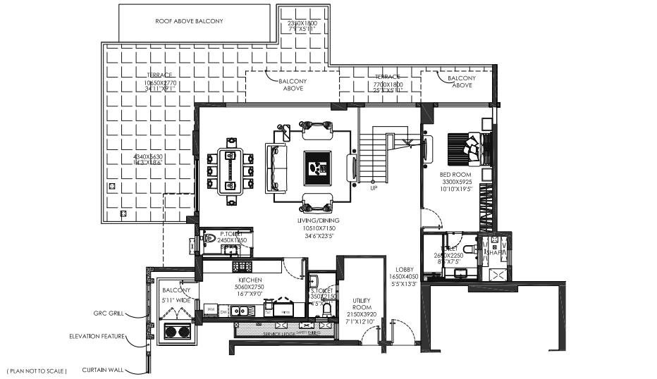
APARTMENT NO. 1 & 2 PENTHOUSE LOWER LEVEL BLOCK F 4969 SQ.FT/ 461.614 SQ.M
