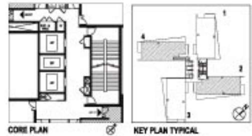
CORE PLAN
