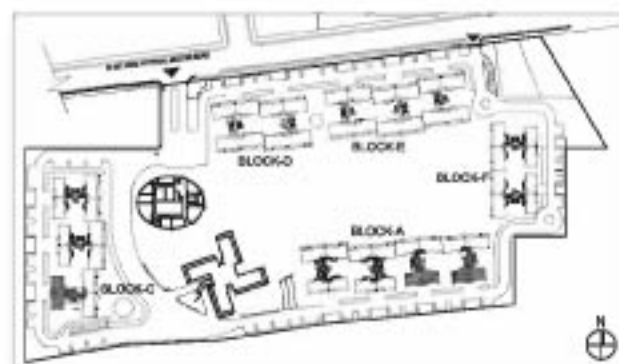
SITE PLAN
