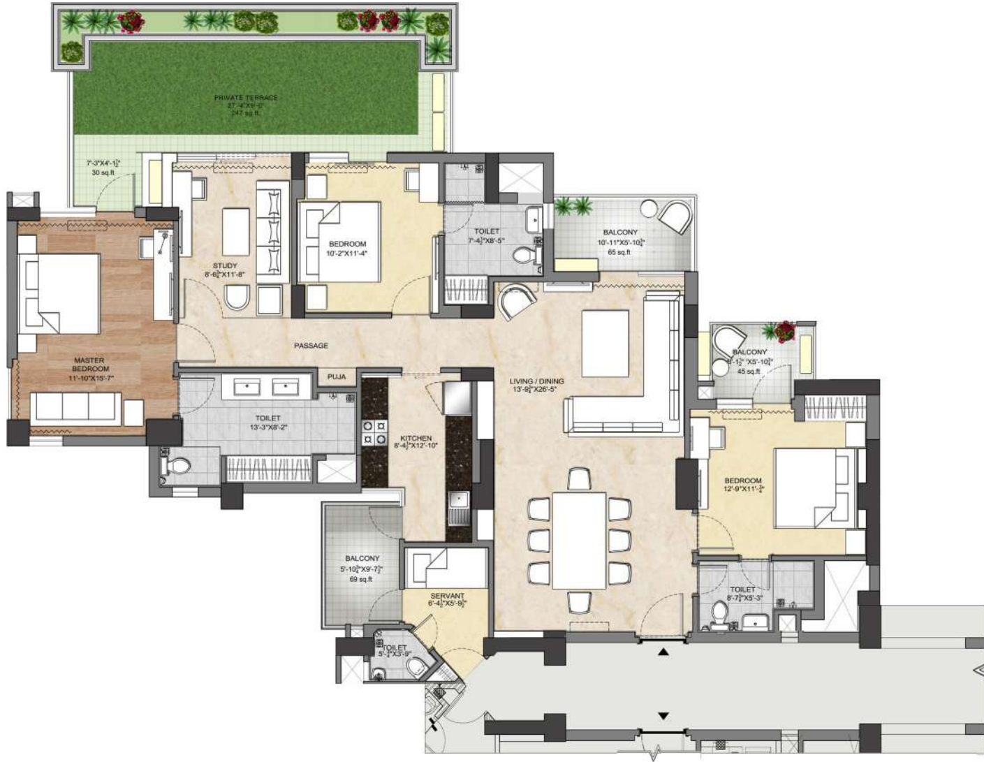
THE TERRACES SIXTH FLOOR UNIT: 3BHK, FAMILY LOUNGE, STUDY, SERVANT ROOM SUPER AREA : 2676.21 SQ.FT
