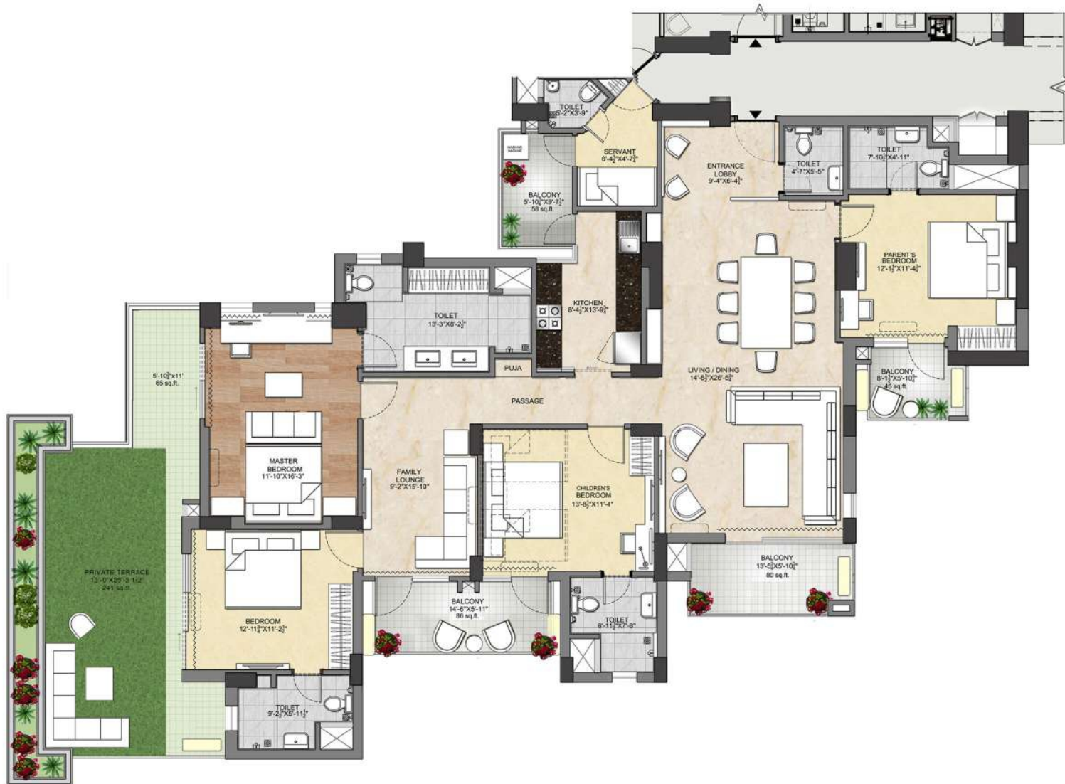
THE TERRACES SECOND FLOOR UNIT: 4BHK, FAMILY LOUNGE, SERVANT ROOM SUPER AREA : 3352.12 SQ.FT.
