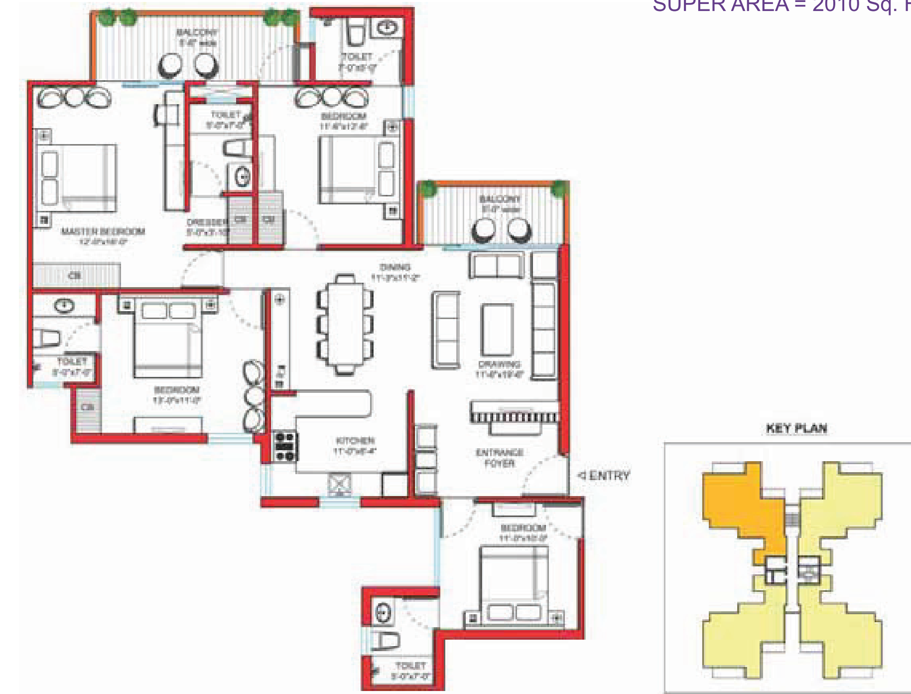
TYPICAL UNIT PLAN 4 BEDROOM UNIT SUPER AREA = 2010 Sq. Ft.
